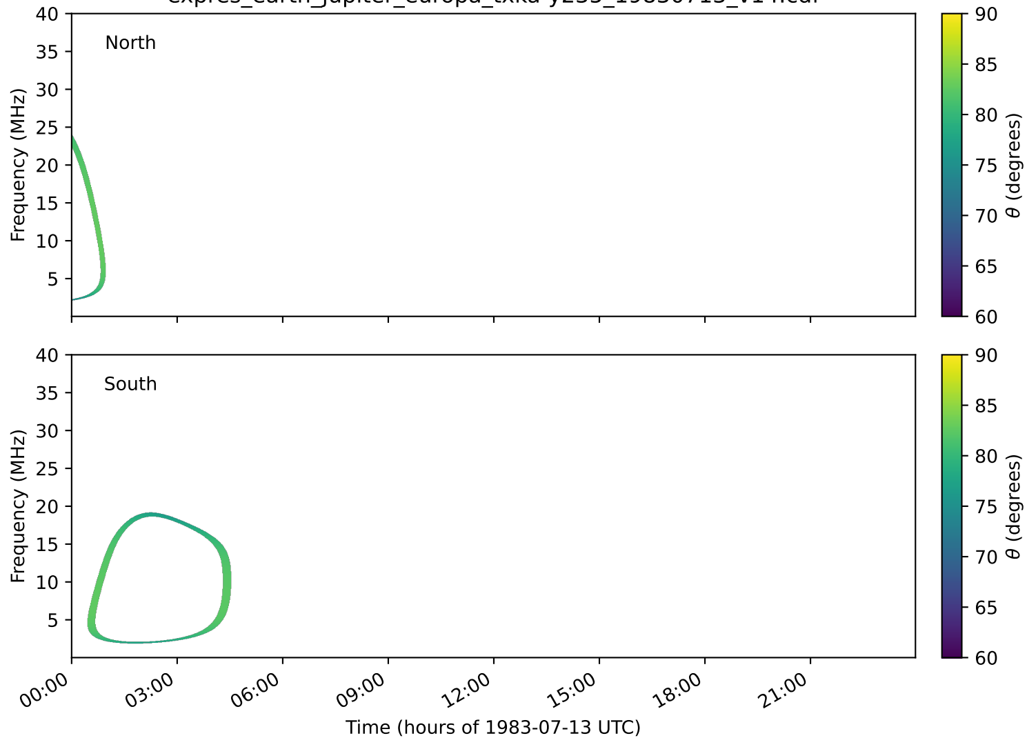
expres_earth_jupiter_europa_txka-y235_19830713_v14.cdf
