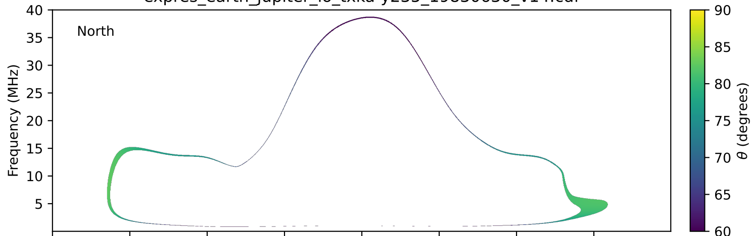
expres_earth_jupiter_io_txka-y235_19830630_v14.cdf
