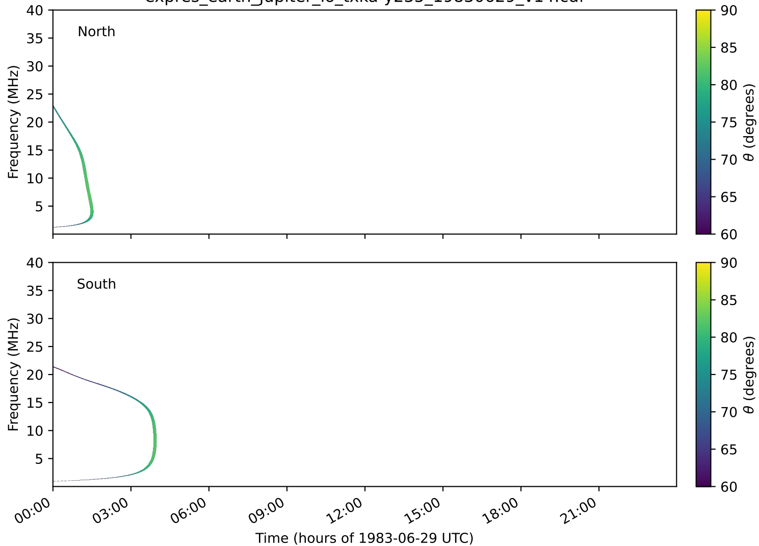
expres_earth_jupiter_io_txka-y235_19830629_v14.cdf
