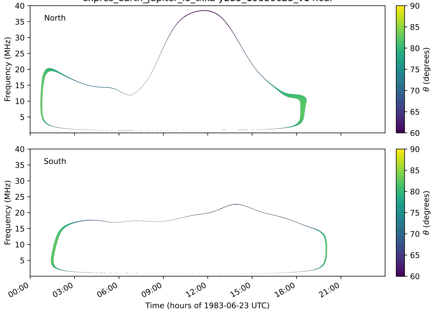
expres_earth_jupiter_io_txka-y235_19830623_v14.cdf
