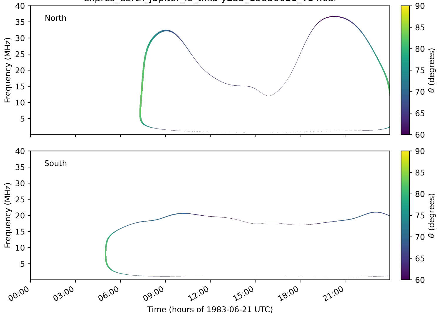
expres_earth_jupiter_io_txka-y235_19830621_v14.cdf
