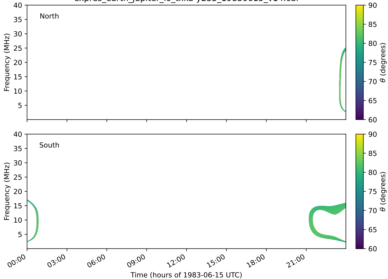
expres_earth_jupiter_io_txka-y235_19830615_v14.cdf
