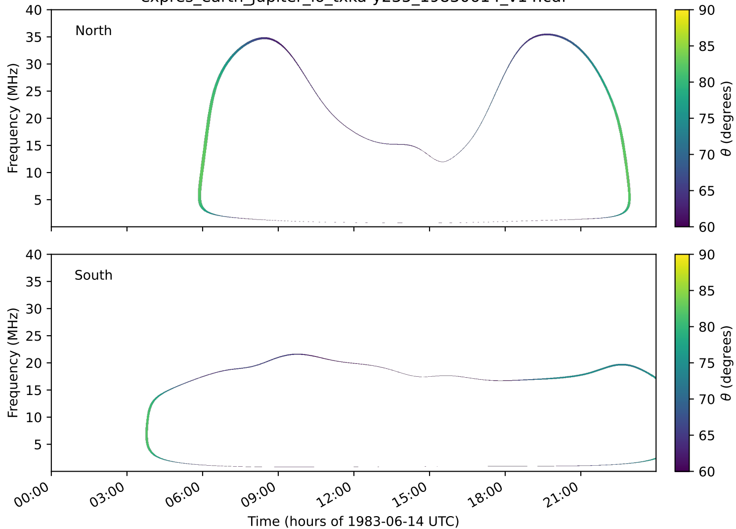
expres_earth_jupiter_io_txka-y235_19830614_v14.cdf
