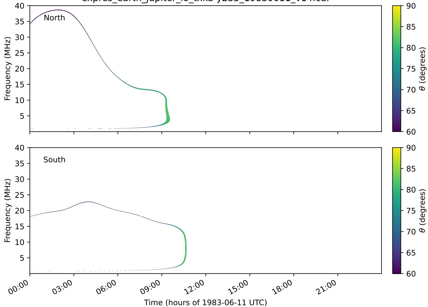
expres_earth_jupiter_io_txka-y235_19830611_v14.cdf
