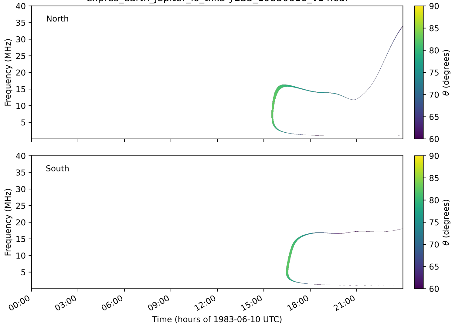
expres_earth_jupiter_io_txka-y235_19830610_v14.cdf
