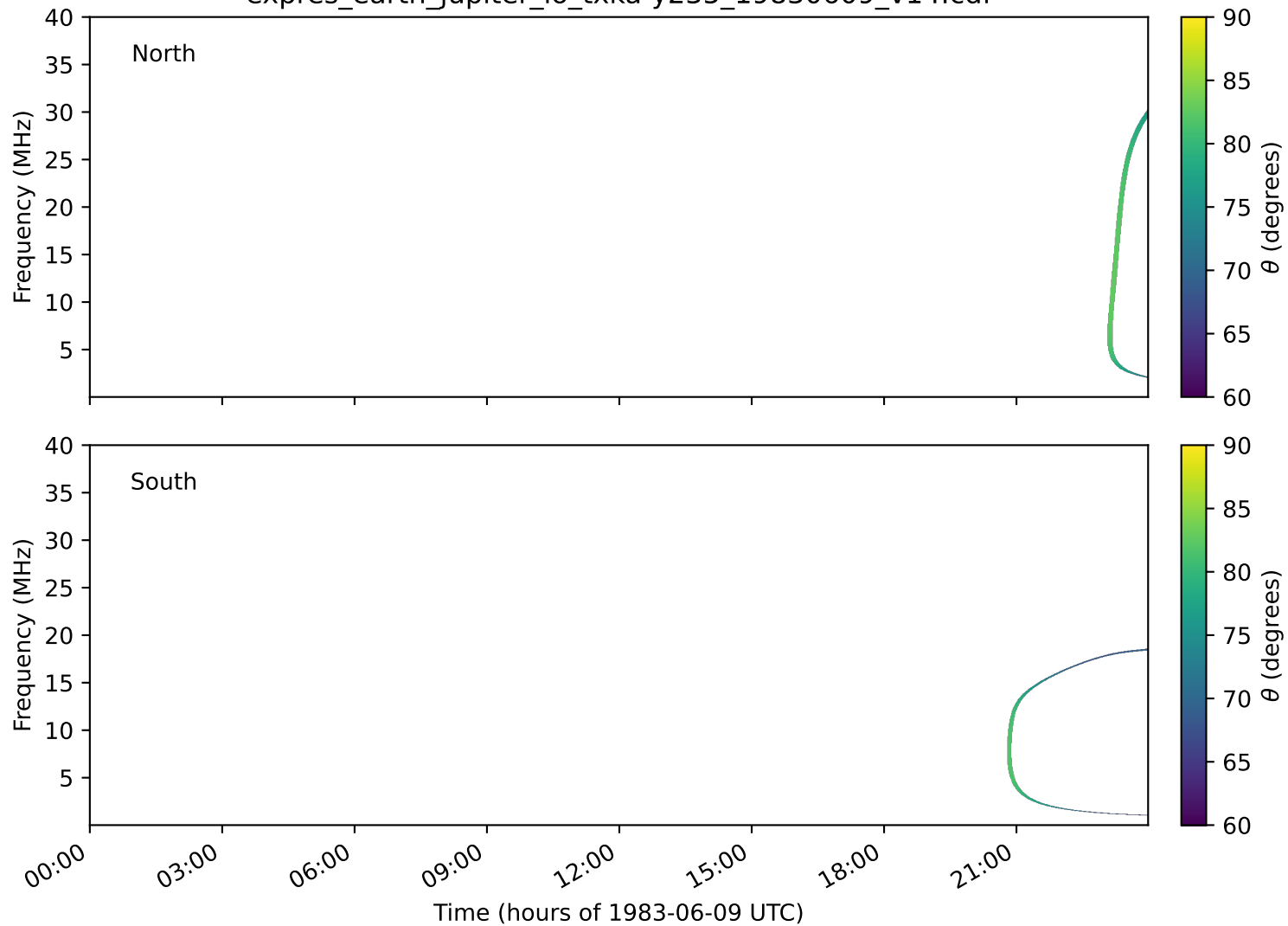
expres_earth_jupiter_io_txka-y235_19830609_v14.cdf
