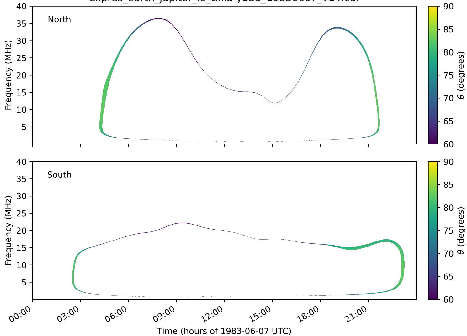
expres_earth_jupiter_io_txka-y235_19830607_v14.cdf
