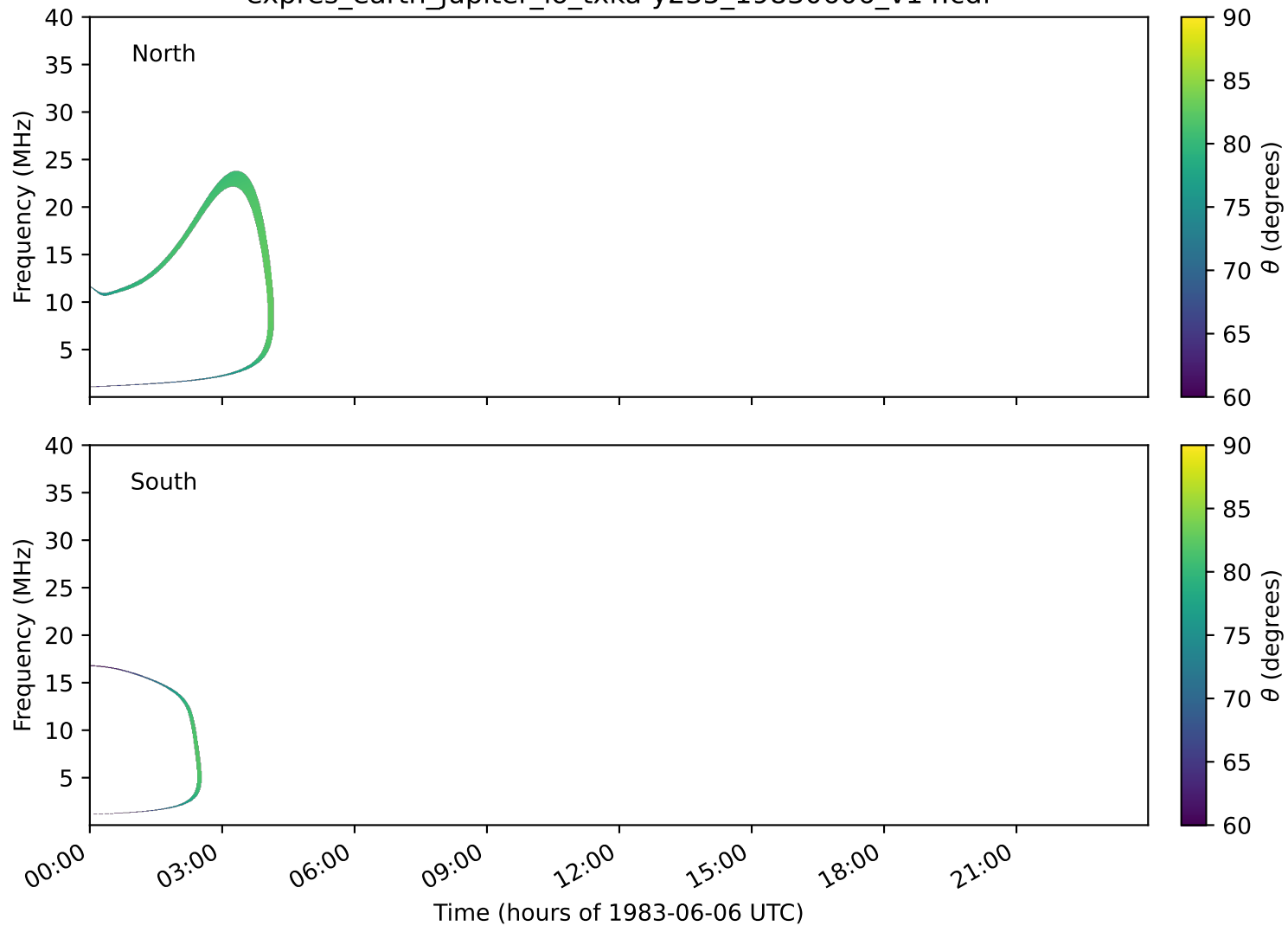
expres_earth_jupiter_io_txka-y235_19830606_v14.cdf
