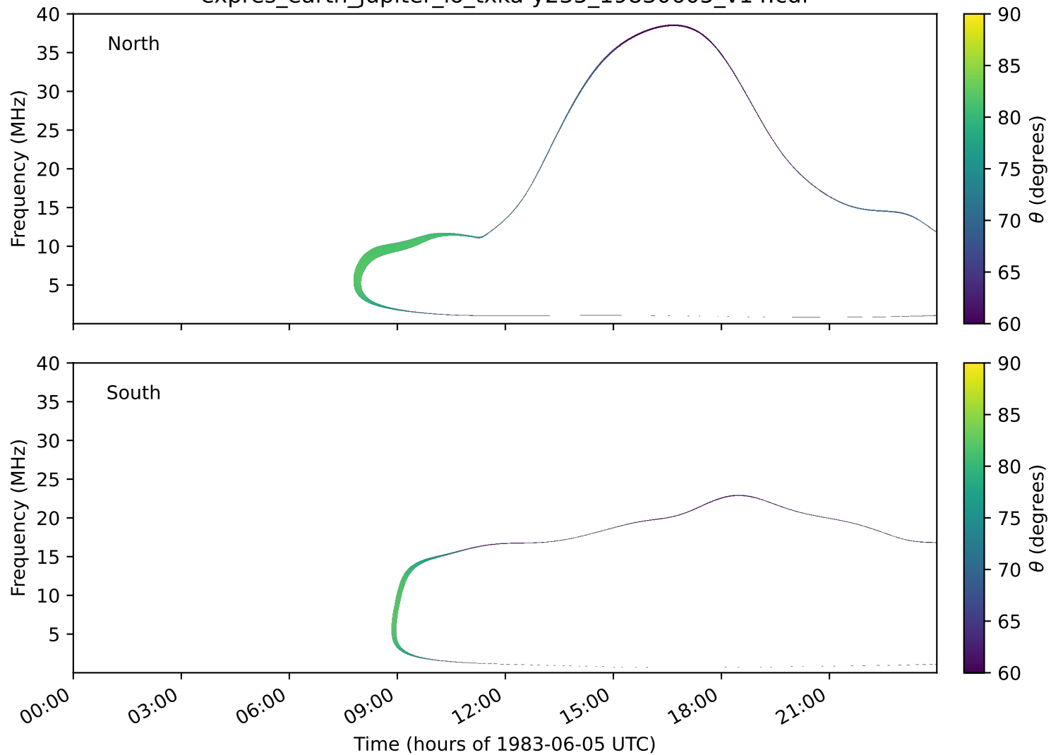
expres_earth_jupiter_io_txka-y235_19830605_v14.cdf
