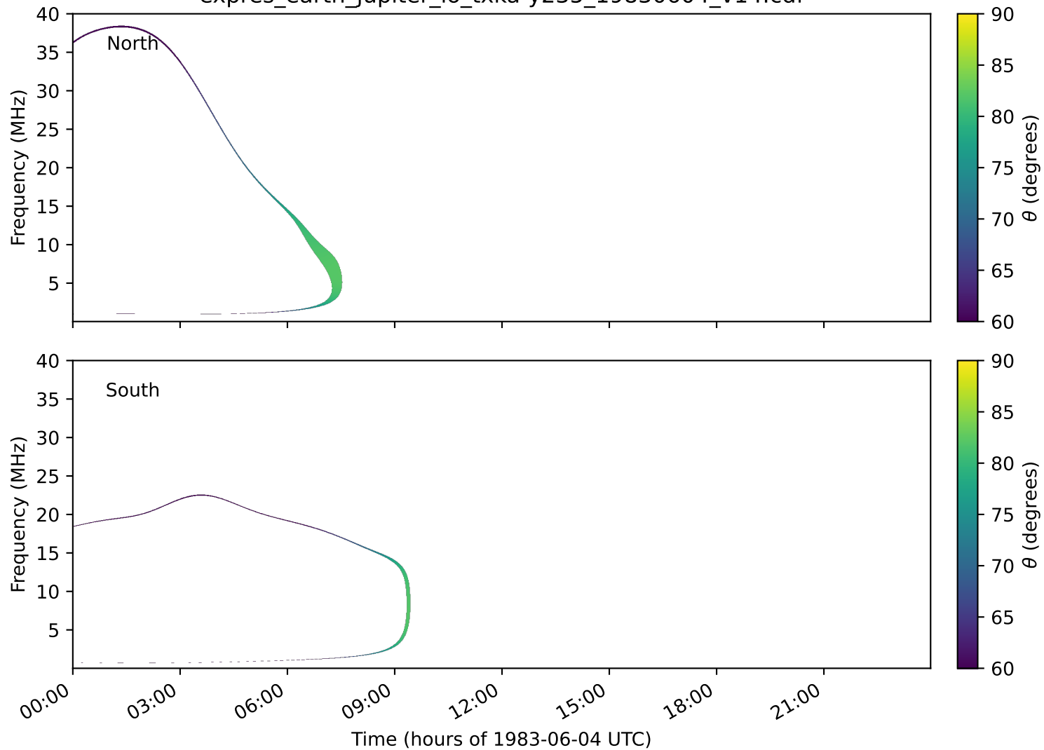
expres_earth_jupiter_io_txka-y235_19830604_v14.cdf
