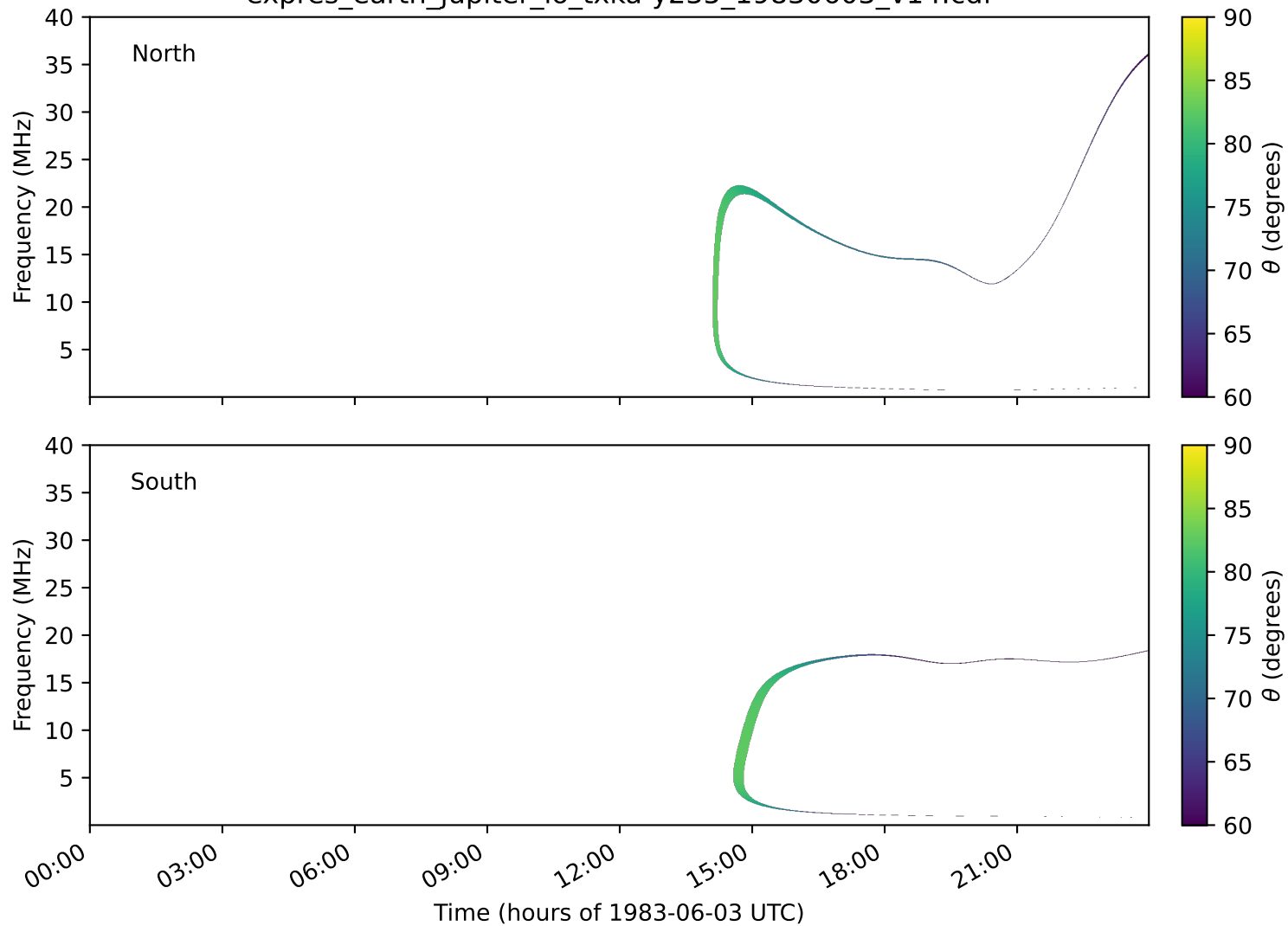
expres_earth_jupiter_io_txka-y235_19830603_v14.cdf
