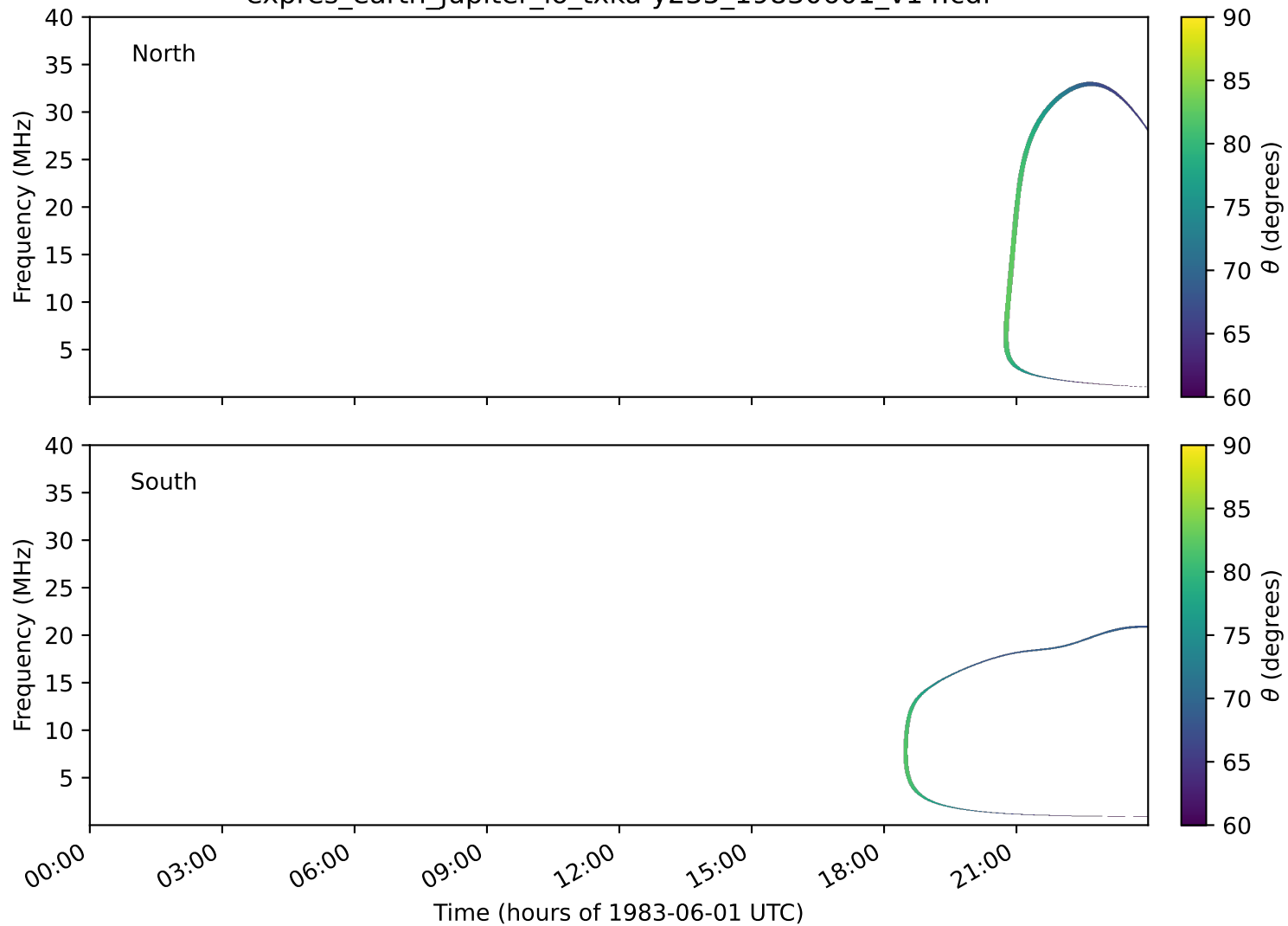
expres_earth_jupiter_io_txka-y235_19830601_v14.cdf
