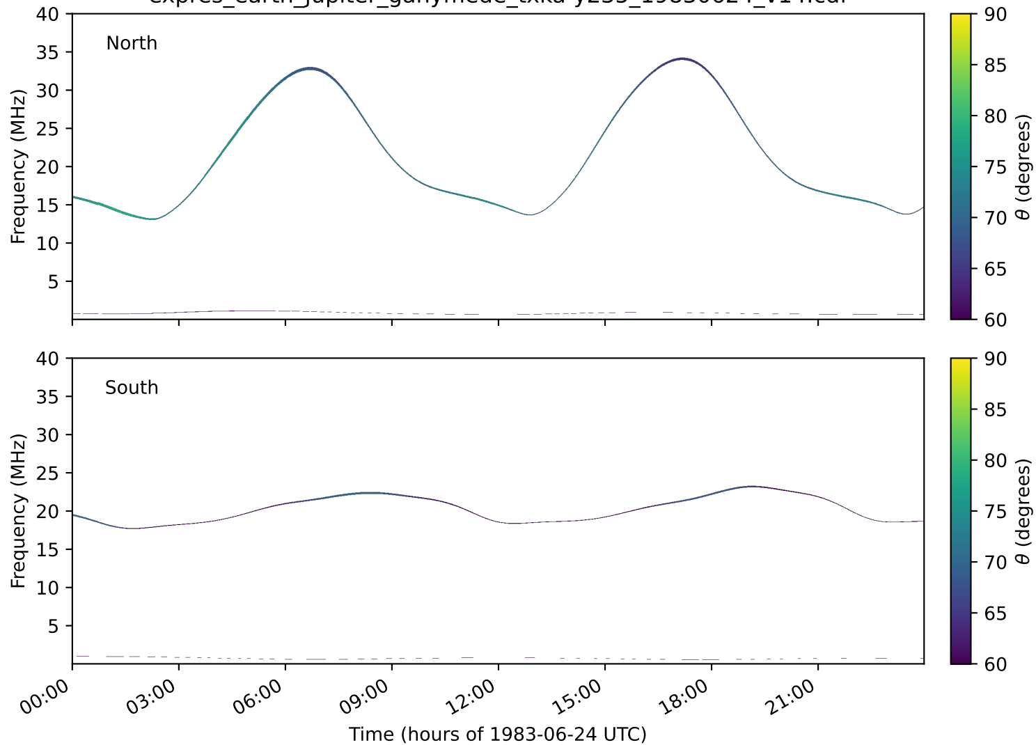
expres_earth_jupiter_ganymede_txka-y235_19830624_v14.cdf
