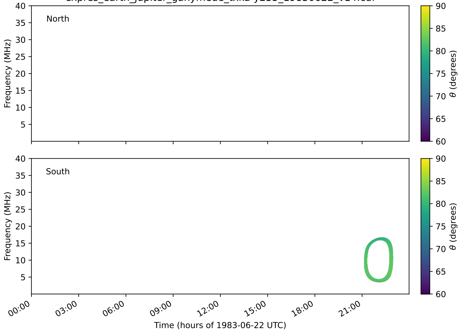
expres_earth_jupiter_ganymede_txka-y235_19830622_v14.cdf
