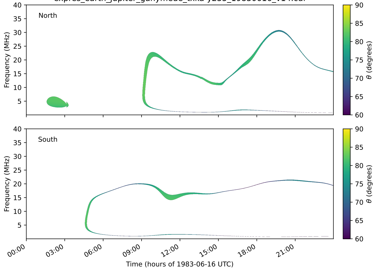
expres_earth_jupiter_ganymede_txka-y235_19830616_v14.cdf
