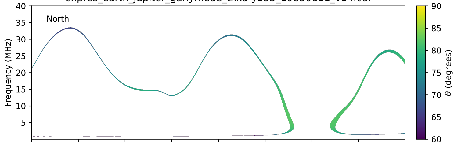
expres_earth_jupiter_ganymede_txka-y235_19830611_v14.cdf
