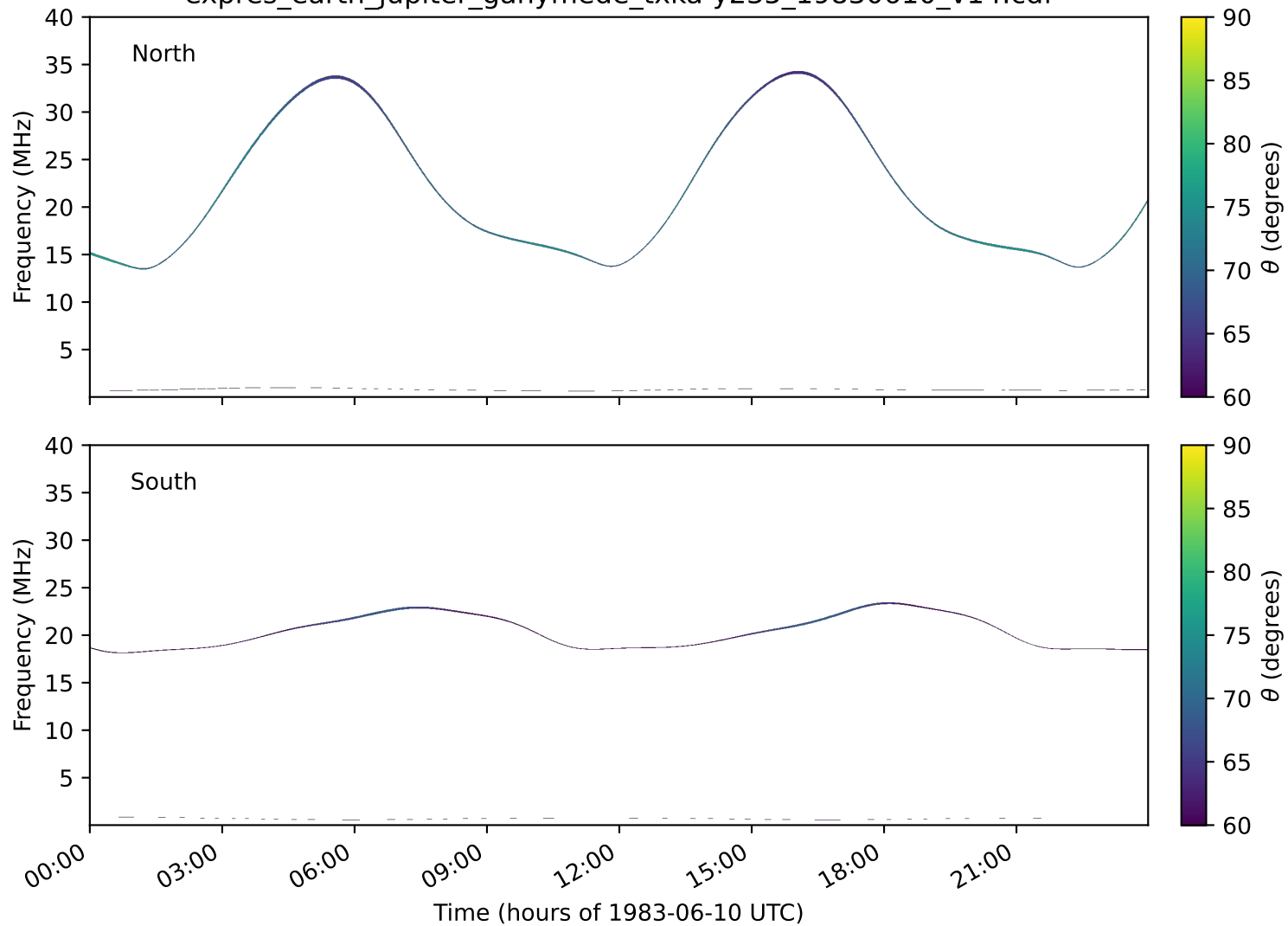
expres_earth_jupiter_ganymede_txka-y235_19830610_v14.cdf
