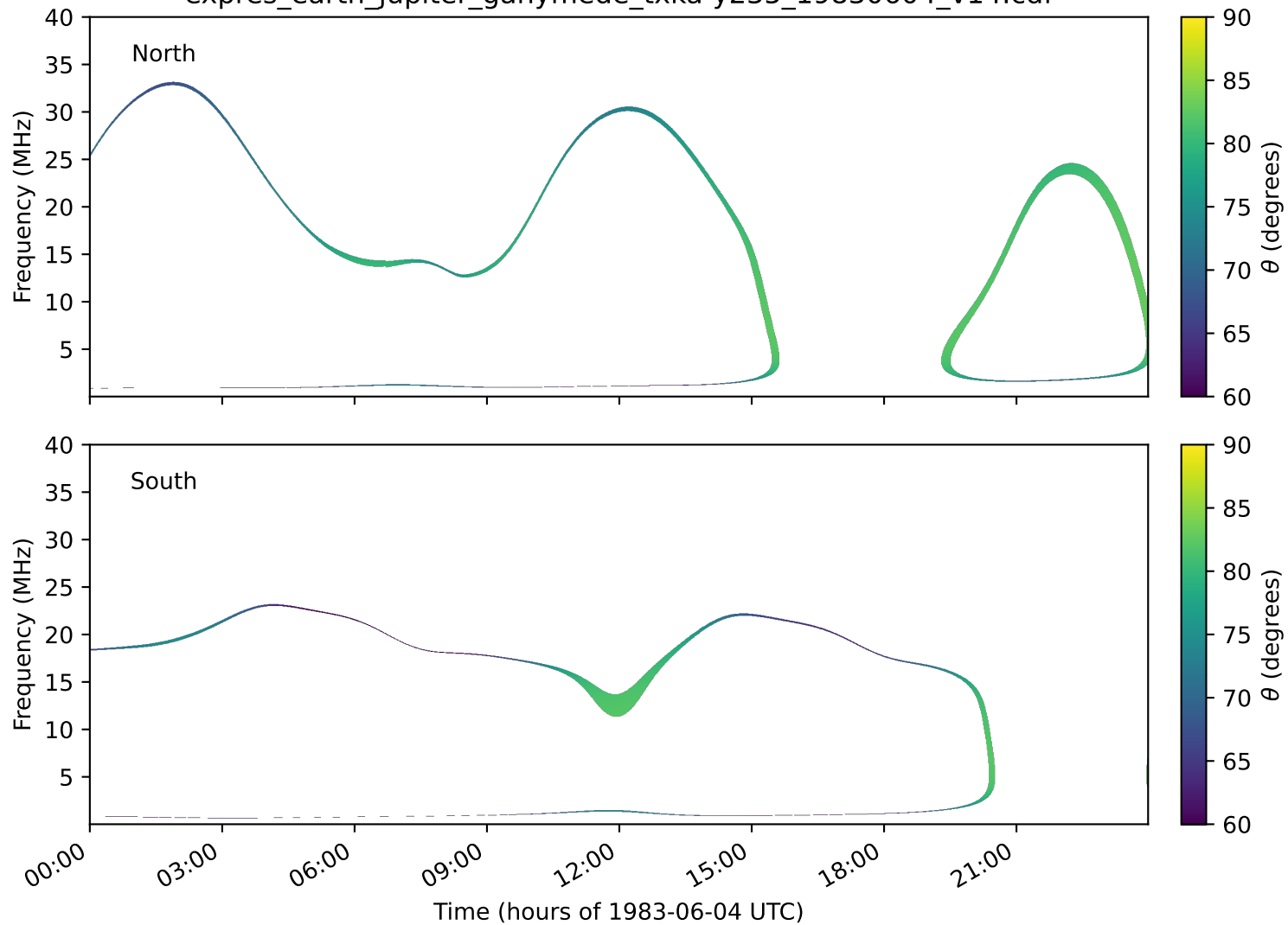
expres_earth_jupiter_ganymede_txka-y235_19830604_v14.cdf
