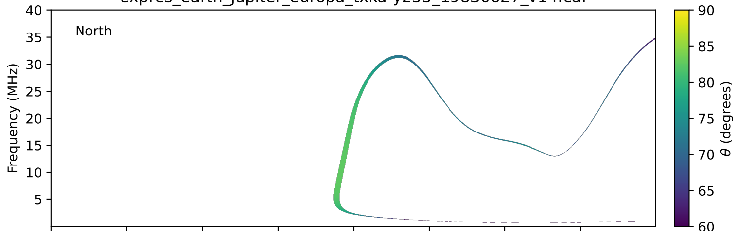
expres_earth_jupiter_europa_txka-y235_19830627_v14.cdf
