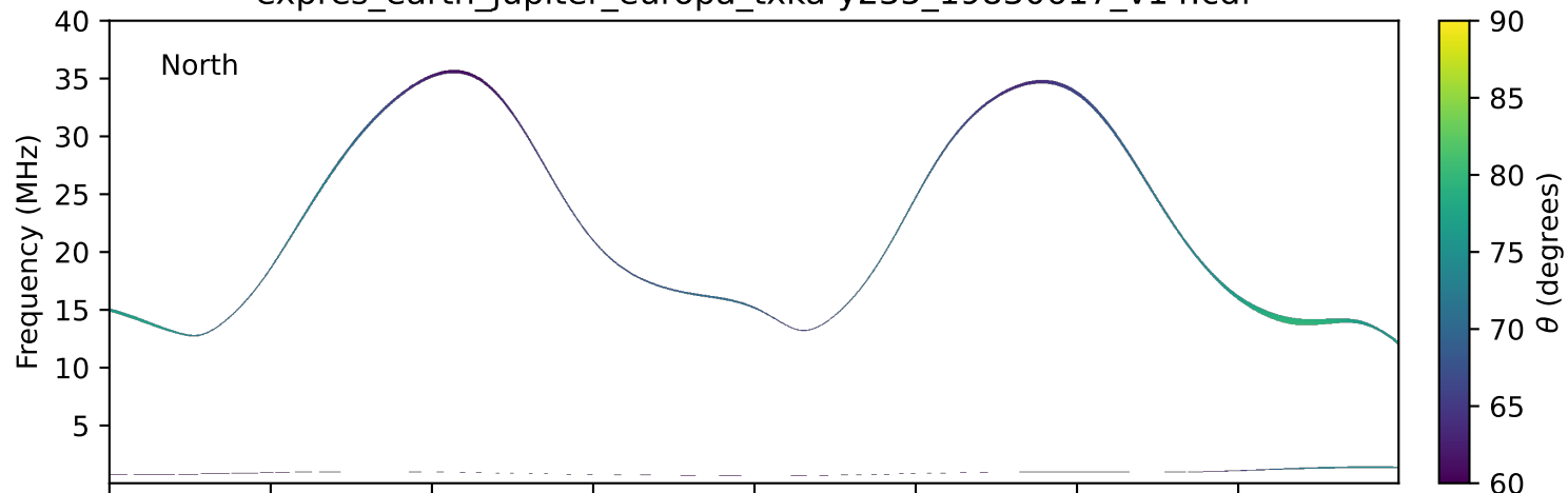
expres_earth_jupiter_europa_txka-y235_19830617_v14.cdf
