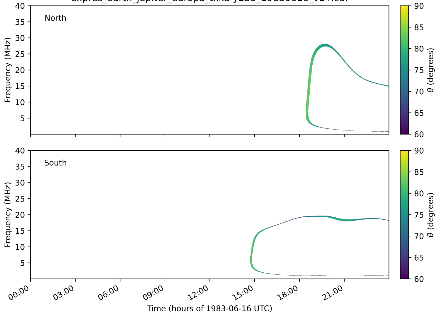
expres_earth_jupiter_europa_txka-y235_19830616_v14.cdf
