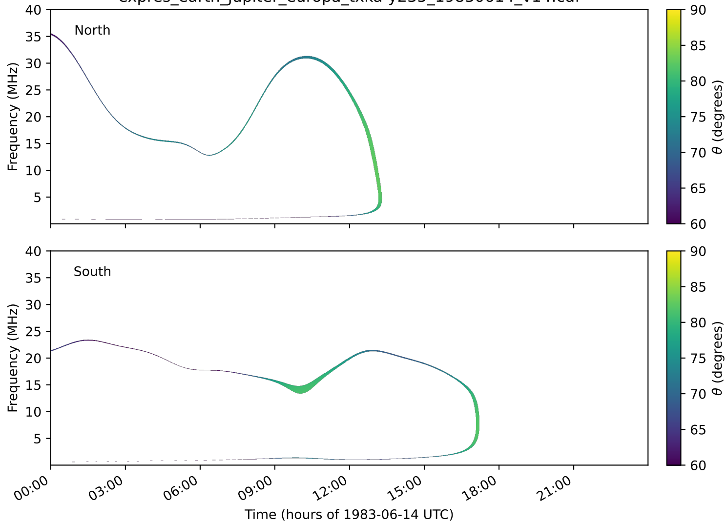
expres_earth_jupiter_europa_txka-y235_19830614_v14.cdf
