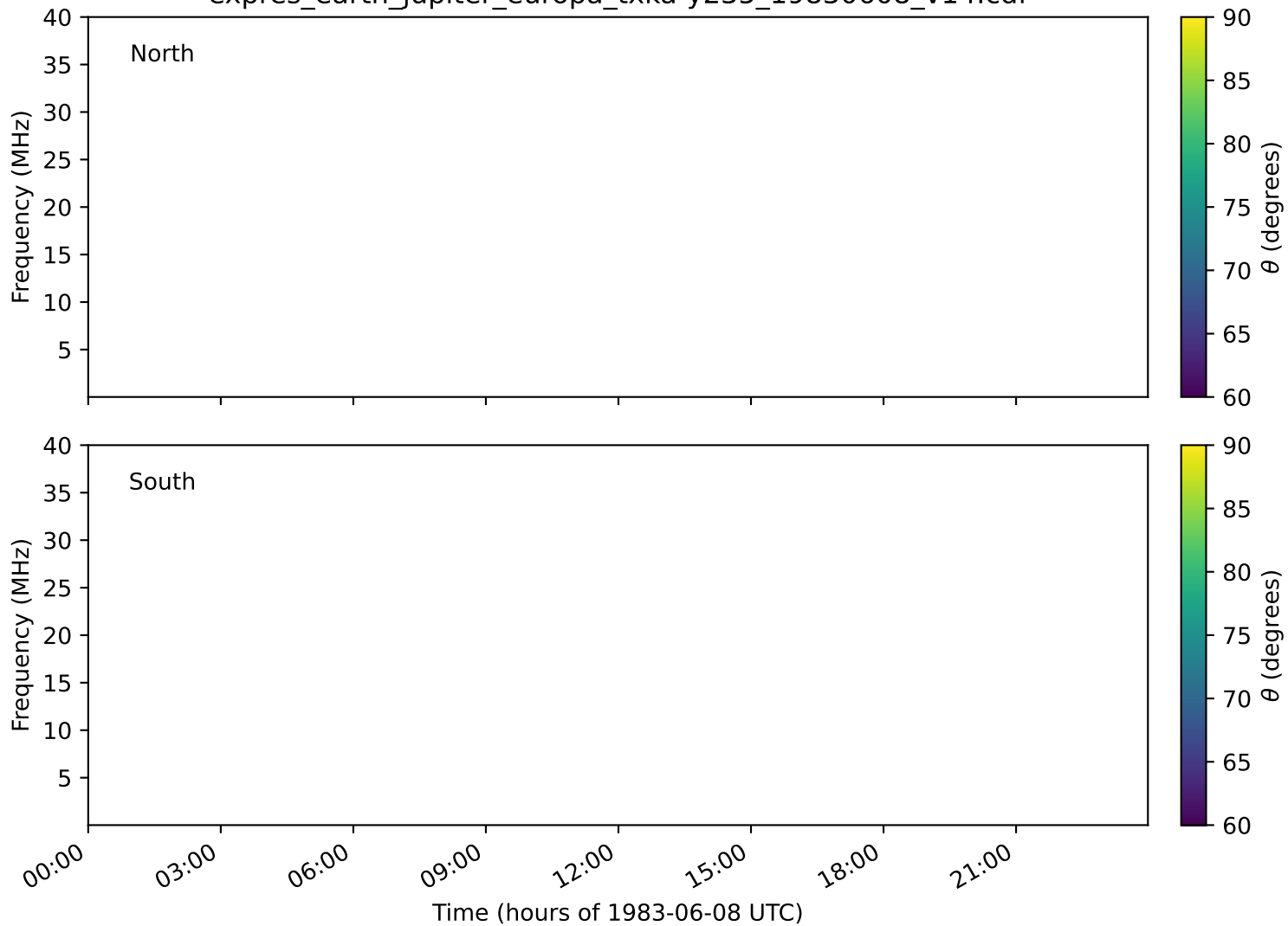
expres_earth_jupiter_europa_txka-y235_19830608_v14.cdf
