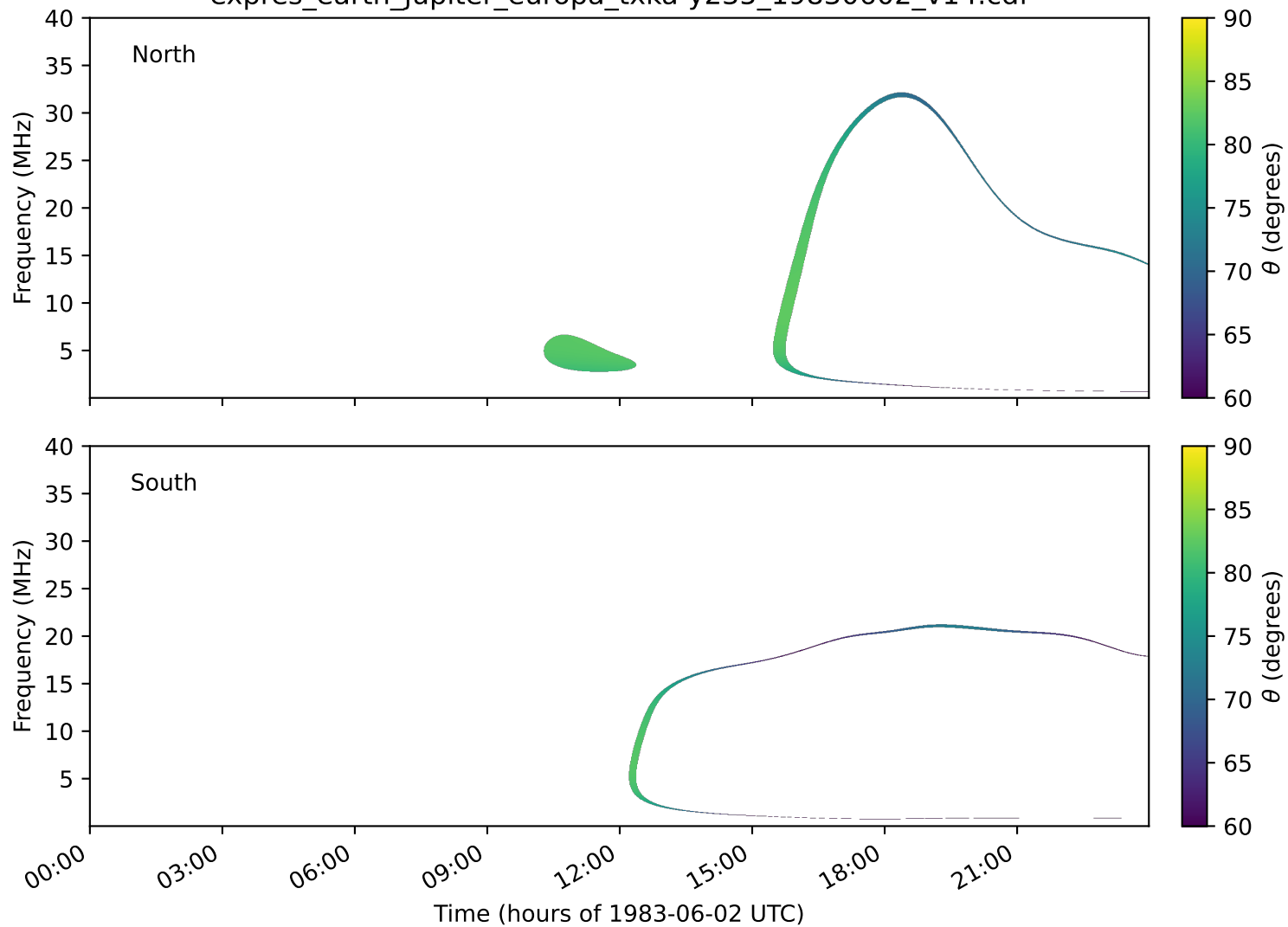
expres_earth_jupiter_europa_txka-y235_19830602_v14.cdf
