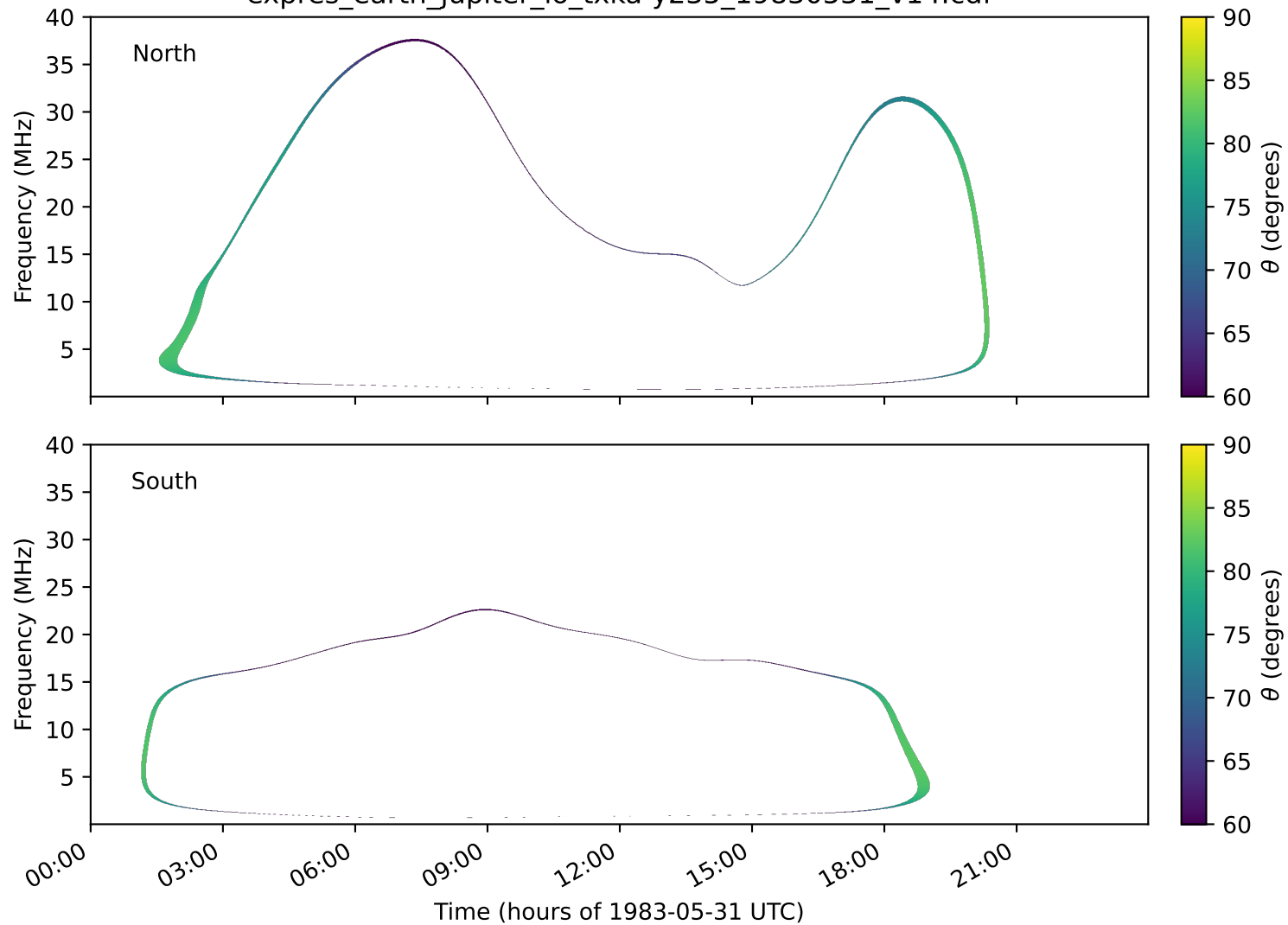
expres_earth_jupiter_io_txka-y235_19830531_v14.cdf
