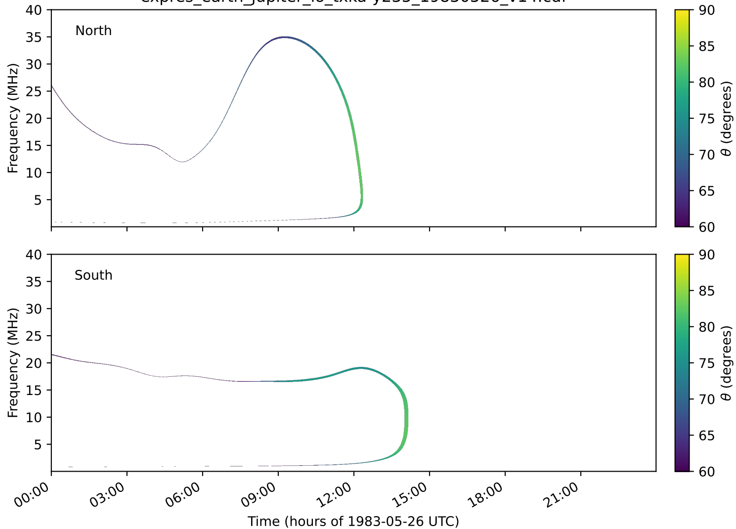
expres_earth_jupiter_io_txka-y235_19830526_v14.cdf
