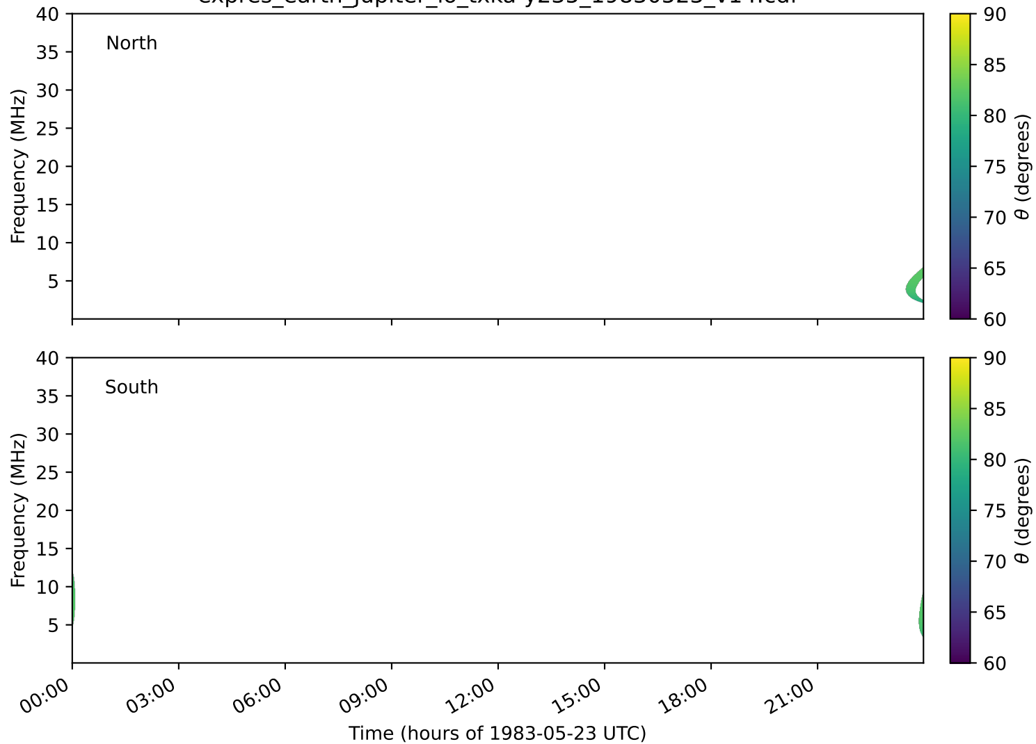
expres_earth_jupiter_io_txka-y235_19830523_v14.cdf
