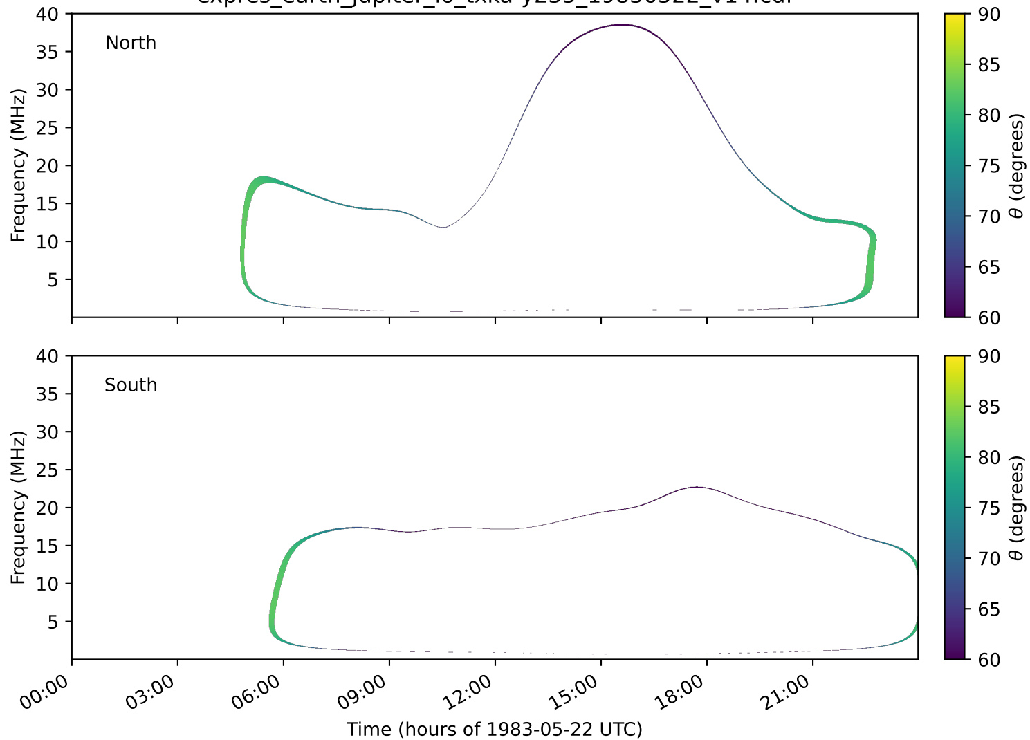
expres_earth_jupiter_io_txka-y235_19830522_v14.cdf
