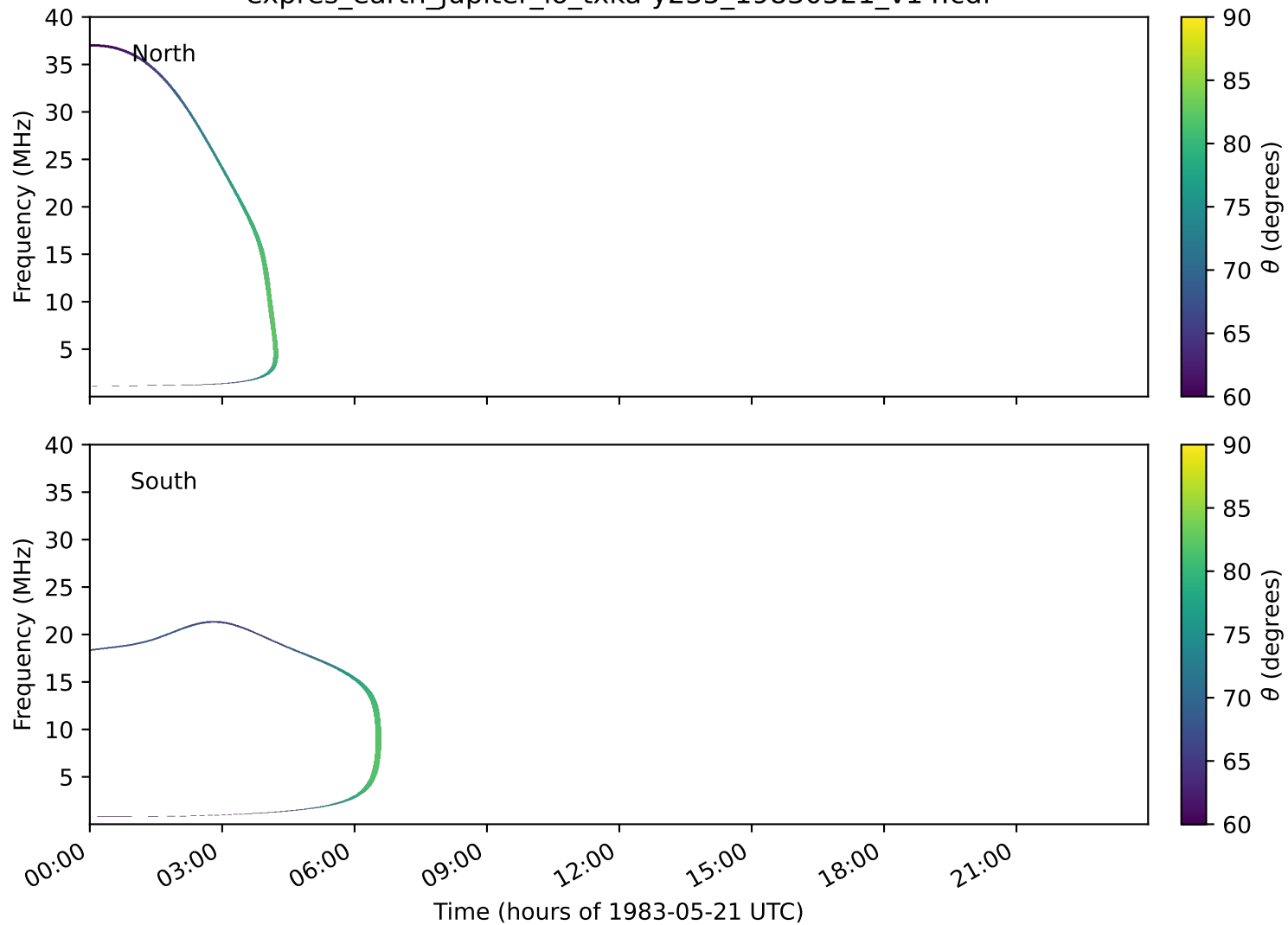
expres_earth_jupiter_io_txka-y235_19830521_v14.cdf
