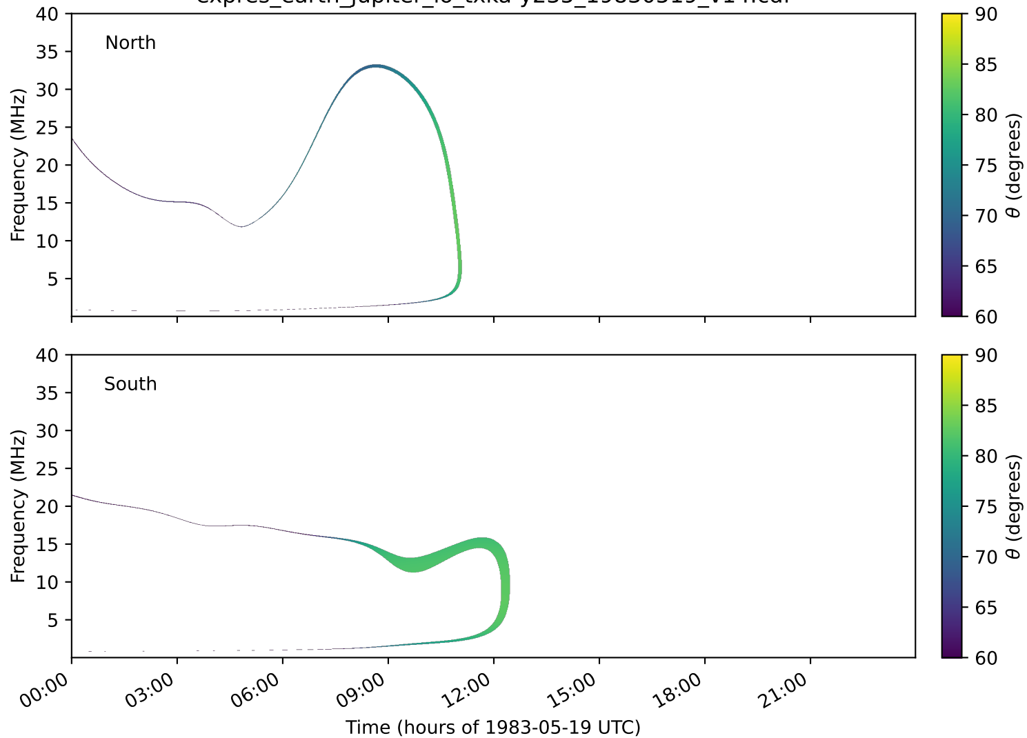
expres_earth_jupiter_io_txka-y235_19830519_v14.cdf
