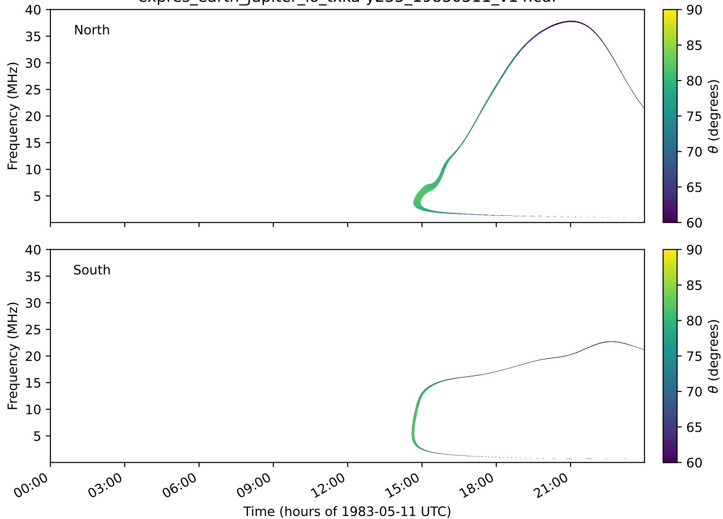
expres_earth_jupiter_io_txka-y235_19830511_v14.cdf
