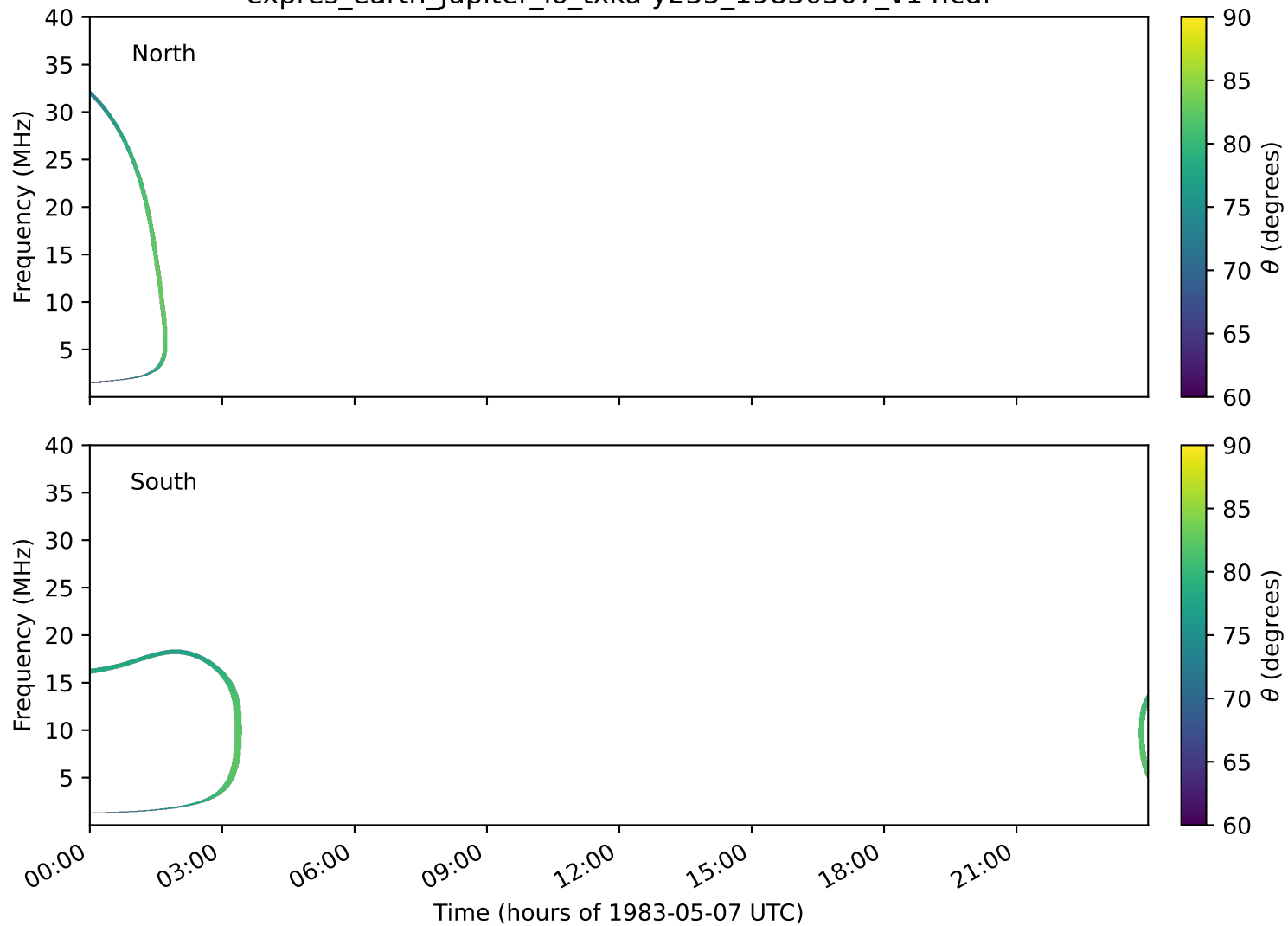
expres_earth_jupiter_io_txka-y235_19830507_v14.cdf
