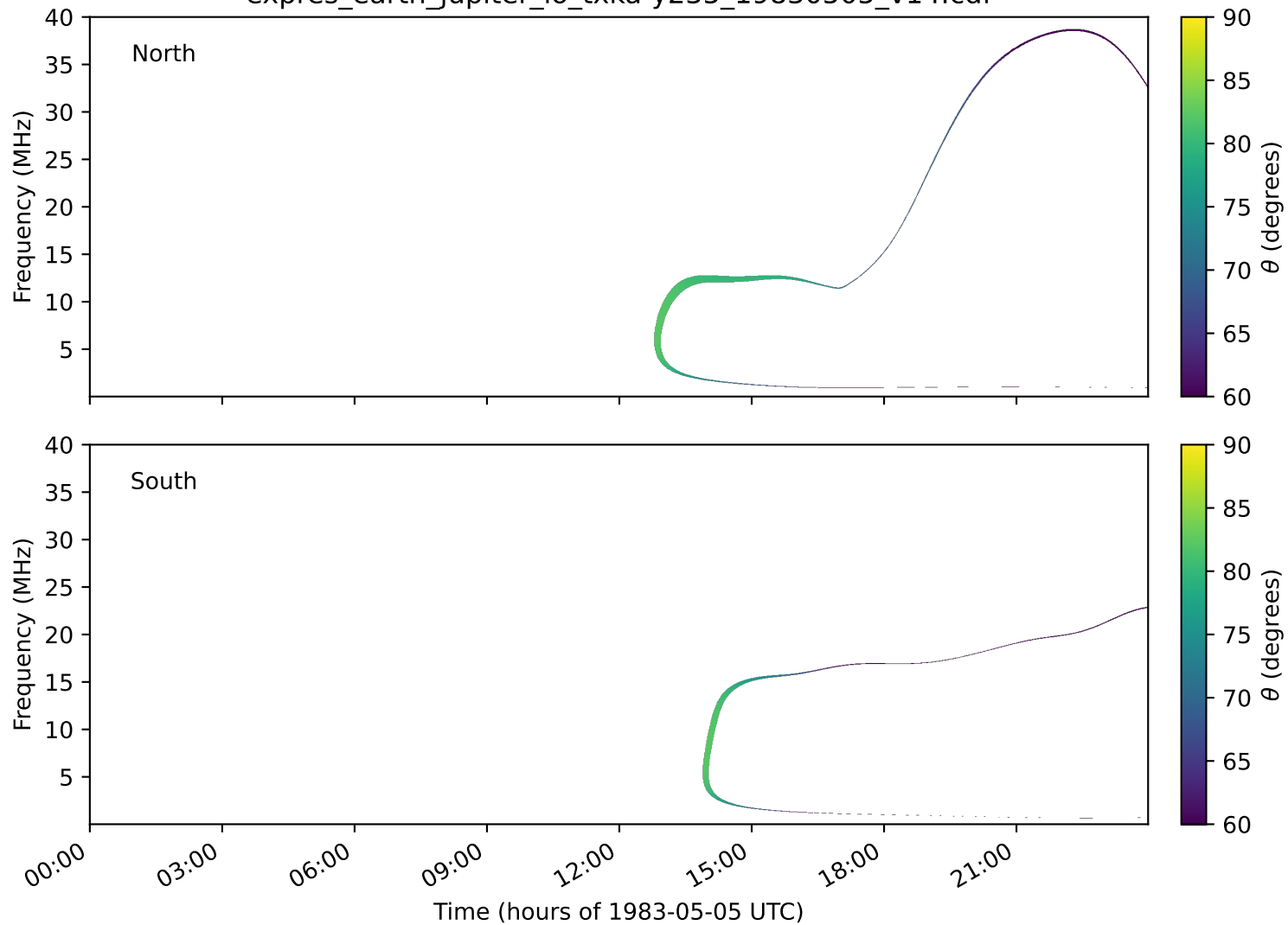
expres_earth_jupiter_io_txka-y235_19830505_v14.cdf
