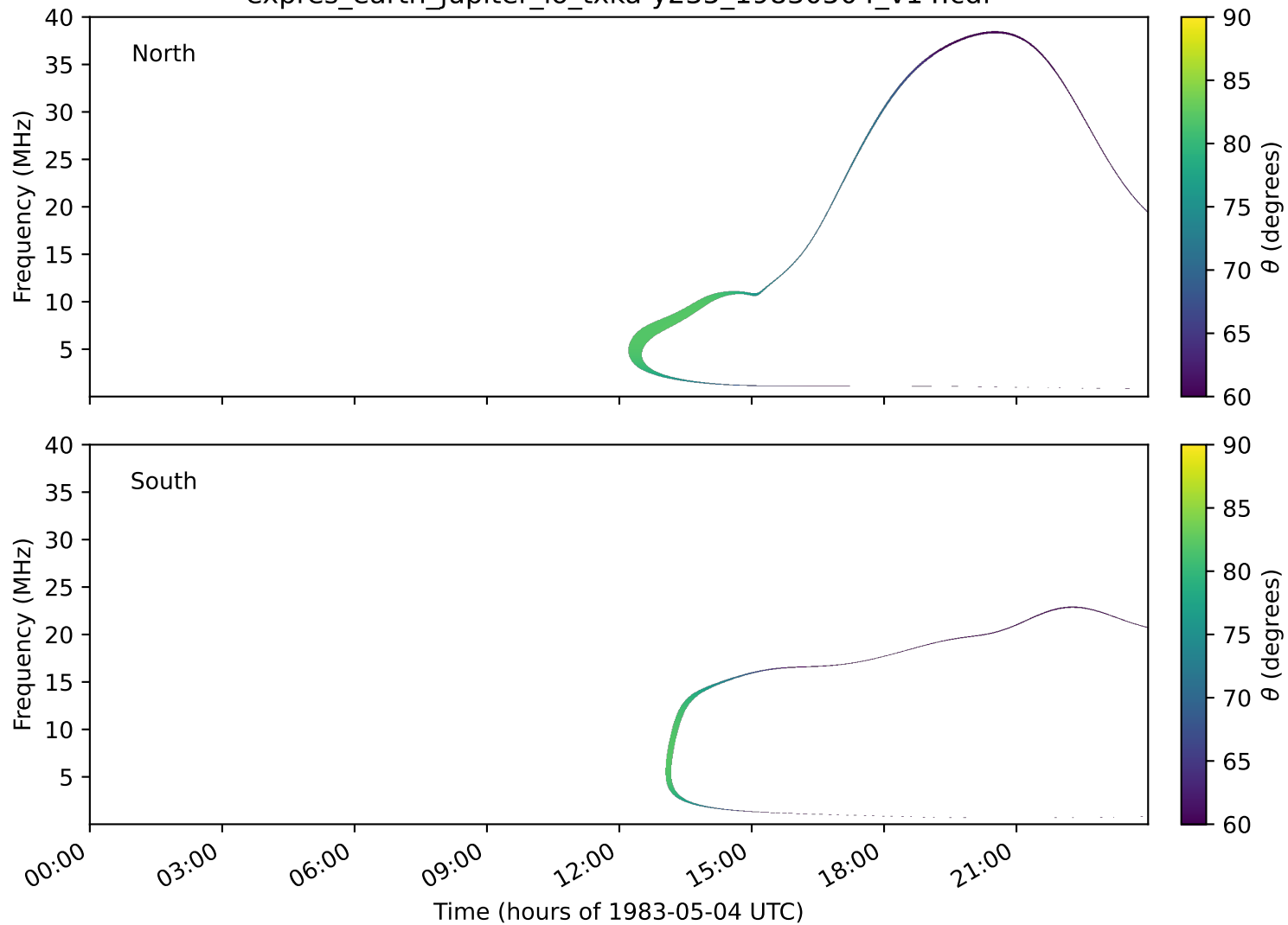
expres_earth_jupiter_io_txka-y235_19830504_v14.cdf
