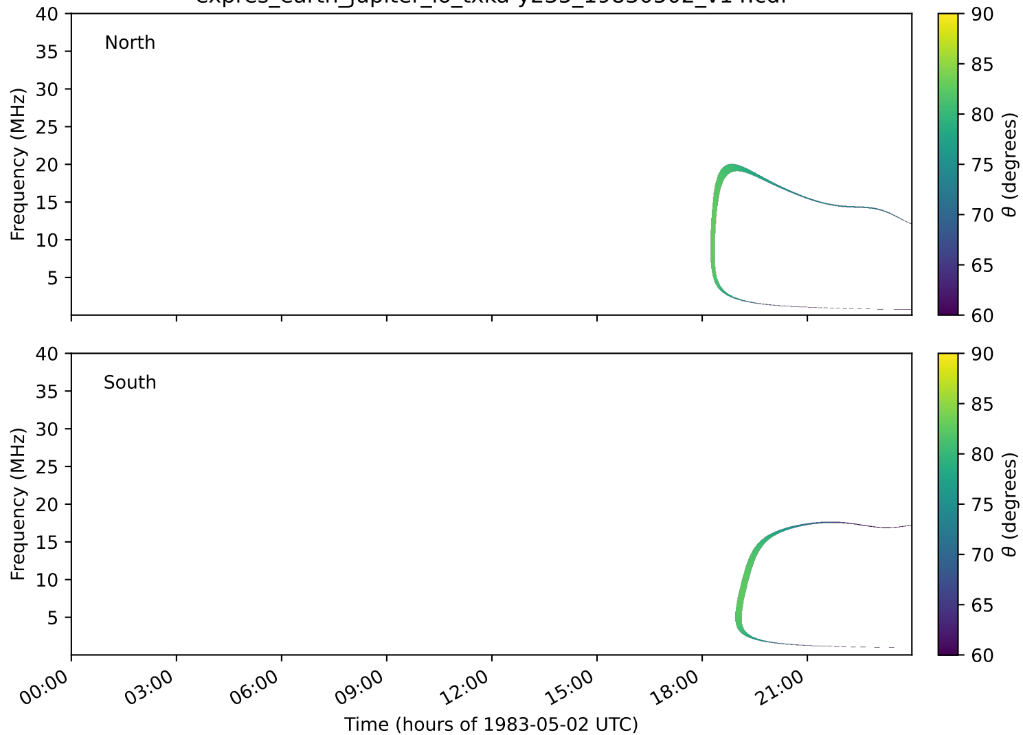
expres_earth_jupiter_io_txka-y235_19830502_v14.cdf
