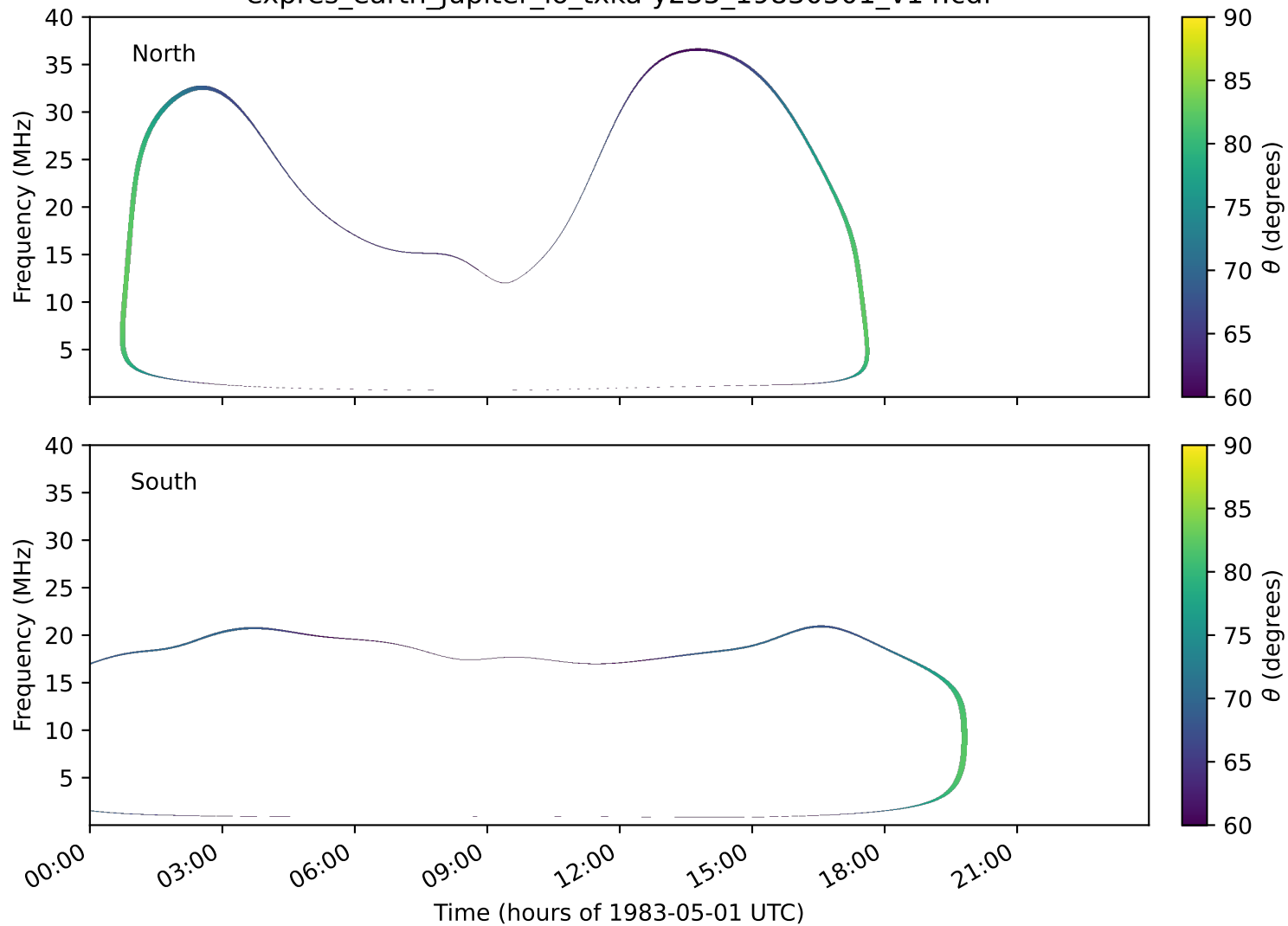
expres_earth_jupiter_io_txka-y235_19830501_v14.cdf
