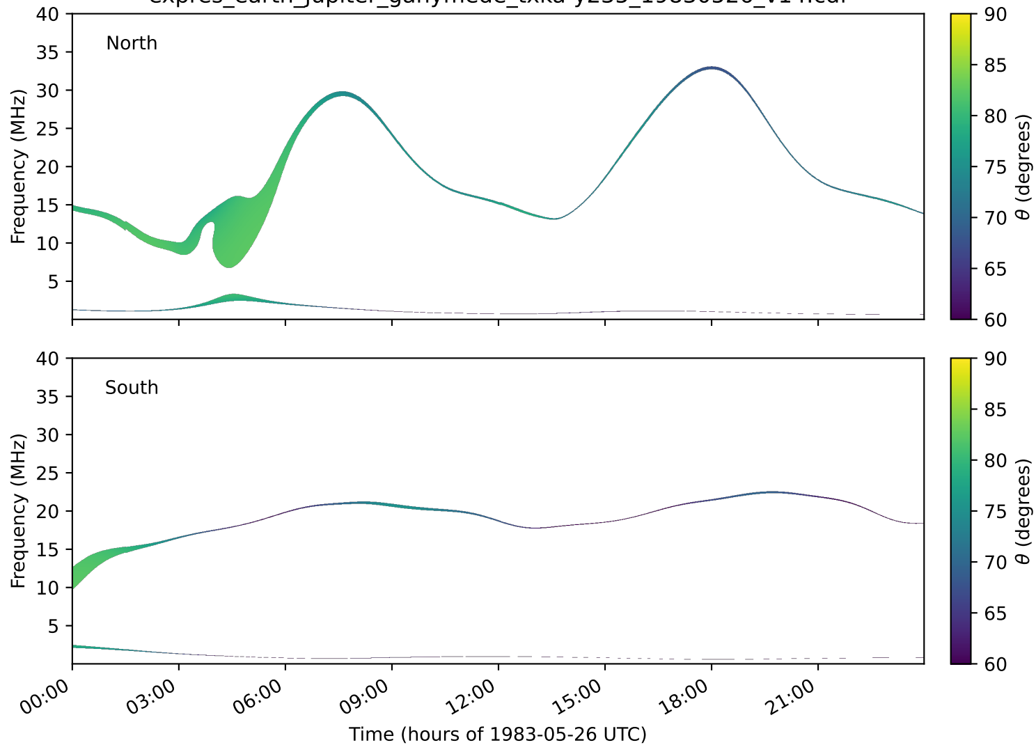
expres_earth_jupiter_ganymede_txka-y235_19830526_v14.cdf
