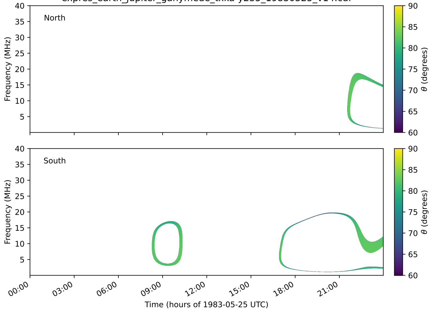
expres_earth_jupiter_ganymede_txka-y235_19830525_v14.cdf
