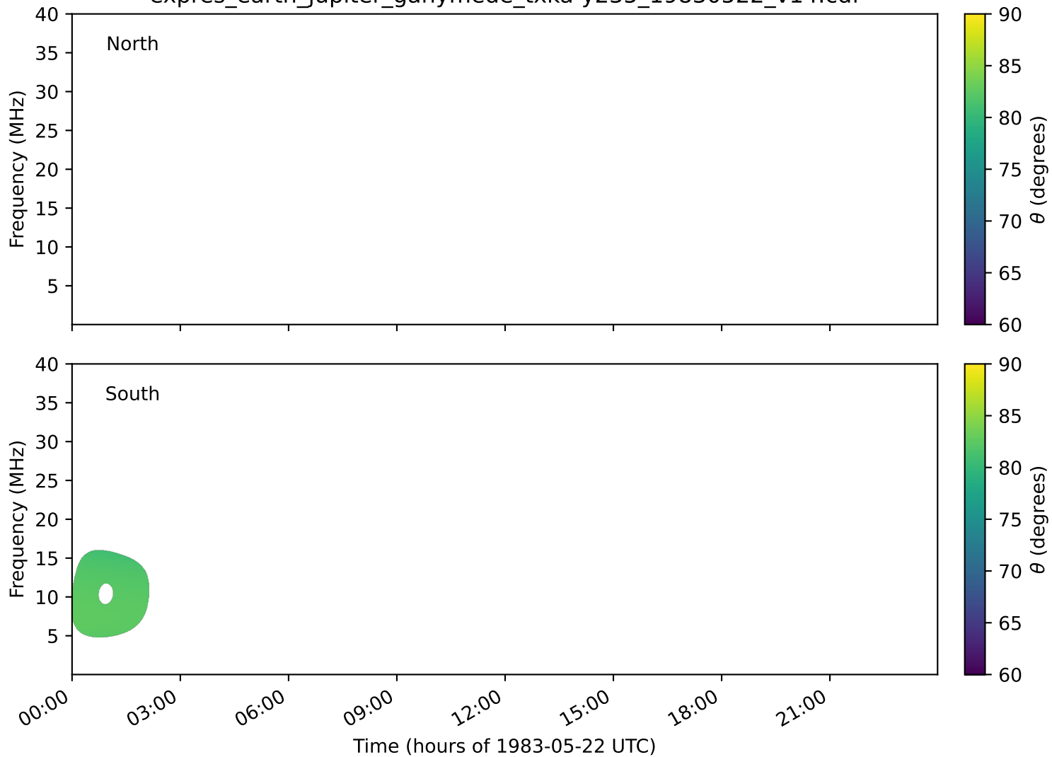
expres_earth_jupiter_ganymede_txka-y235_19830522_v14.cdf
