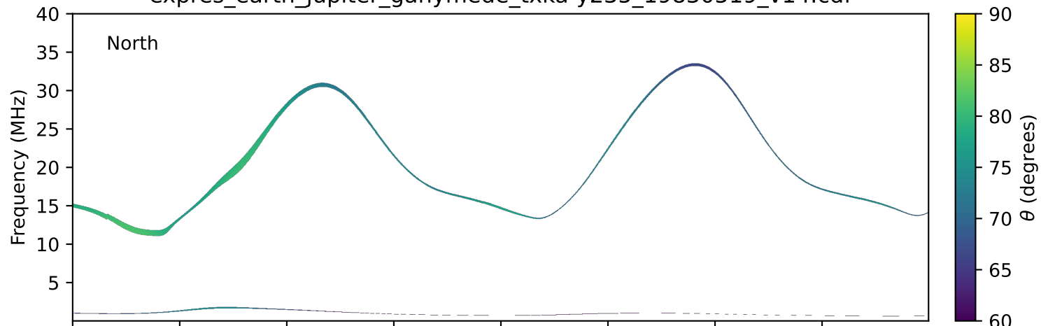
expres_earth_jupiter_ganymede_txka-y235_19830519_v14.cdf
