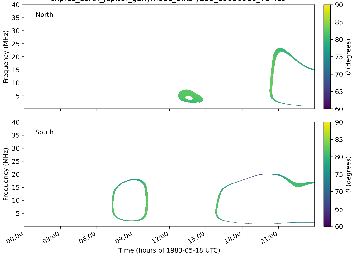
expres_earth_jupiter_ganymede_txka-y235_19830518_v14.cdf
