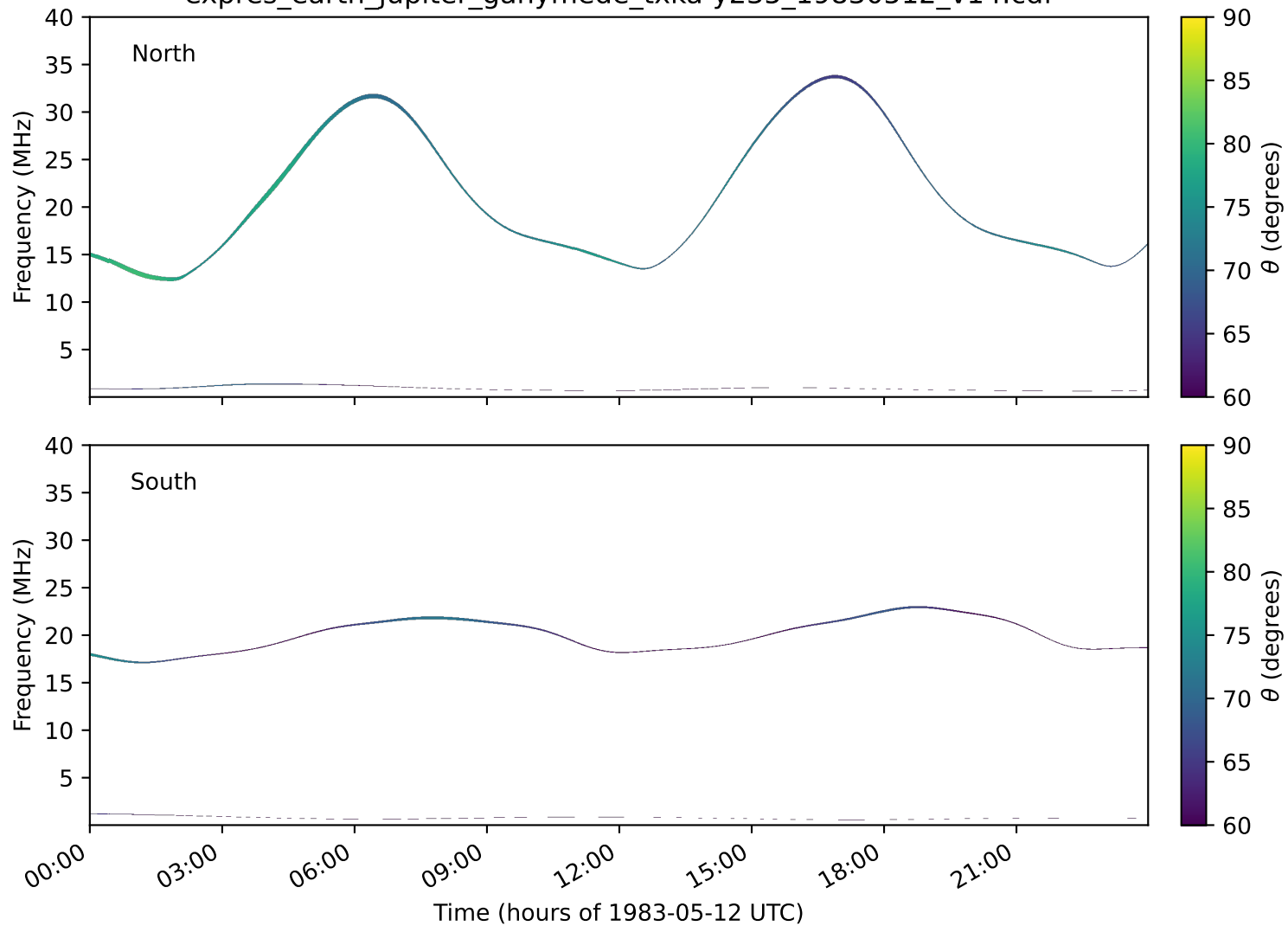
expres_earth_jupiter_ganymede_txka-y235_19830512_v14.cdf
