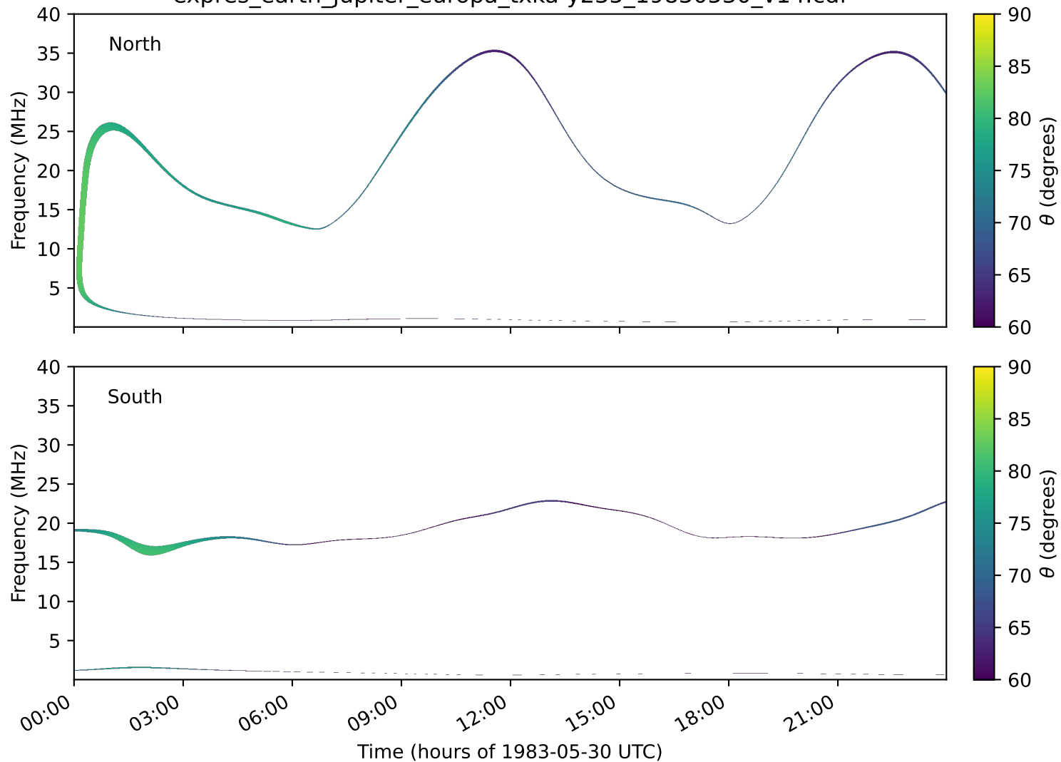
expres_earth_jupiter_europa_txka-y235_19830530_v14.cdf
