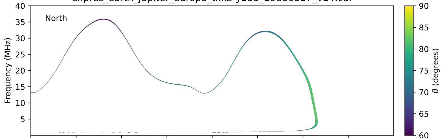
expres_earth_jupiter_europa_txka-y235_19830527_v14.cdf
