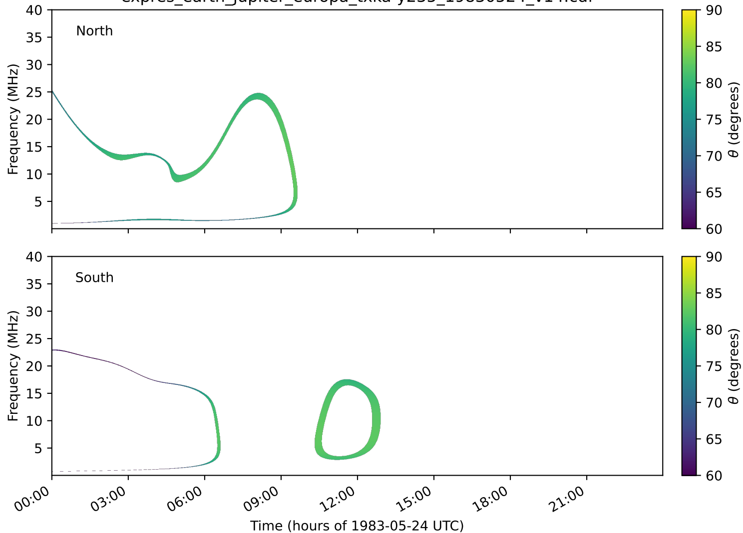
expres_earth_jupiter_europa_txka-y235_19830524_v14.cdf
