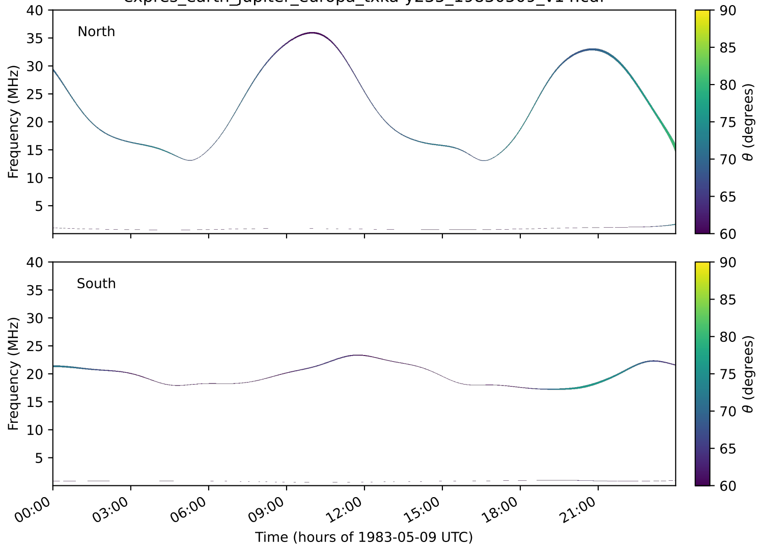
expres_earth_jupiter_europa_txka-y235_19830509_v14.cdf
